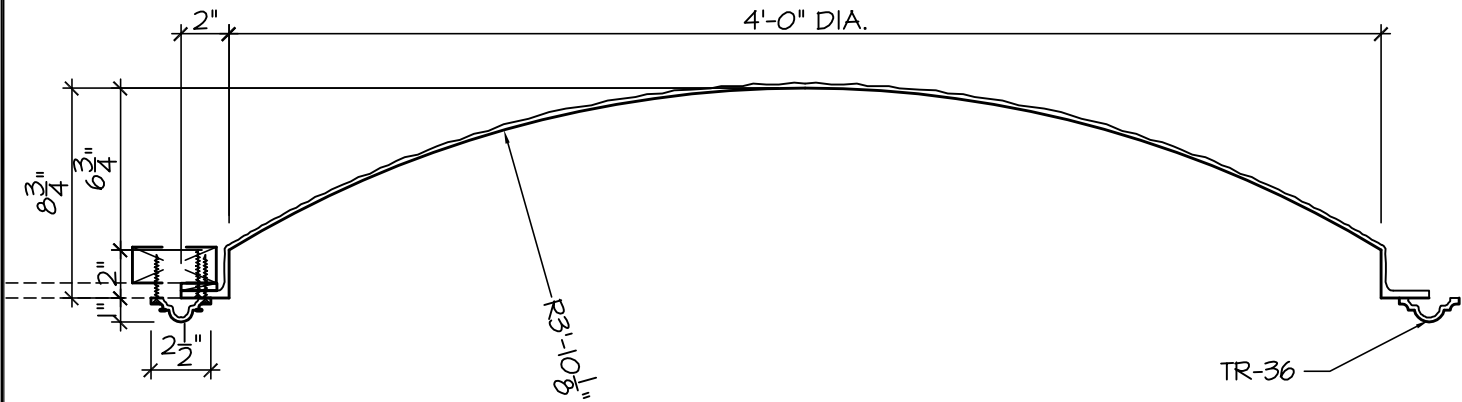
1B DETAIL SECTION SCALE : 1-1/2" = 1'-0"
