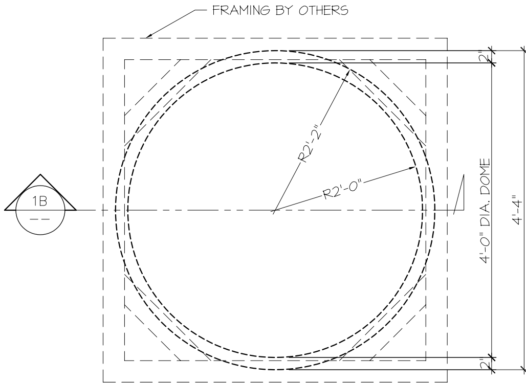
1A REFLECTED PLAN VIEW SCALE : 3/4" = 1'-0"
