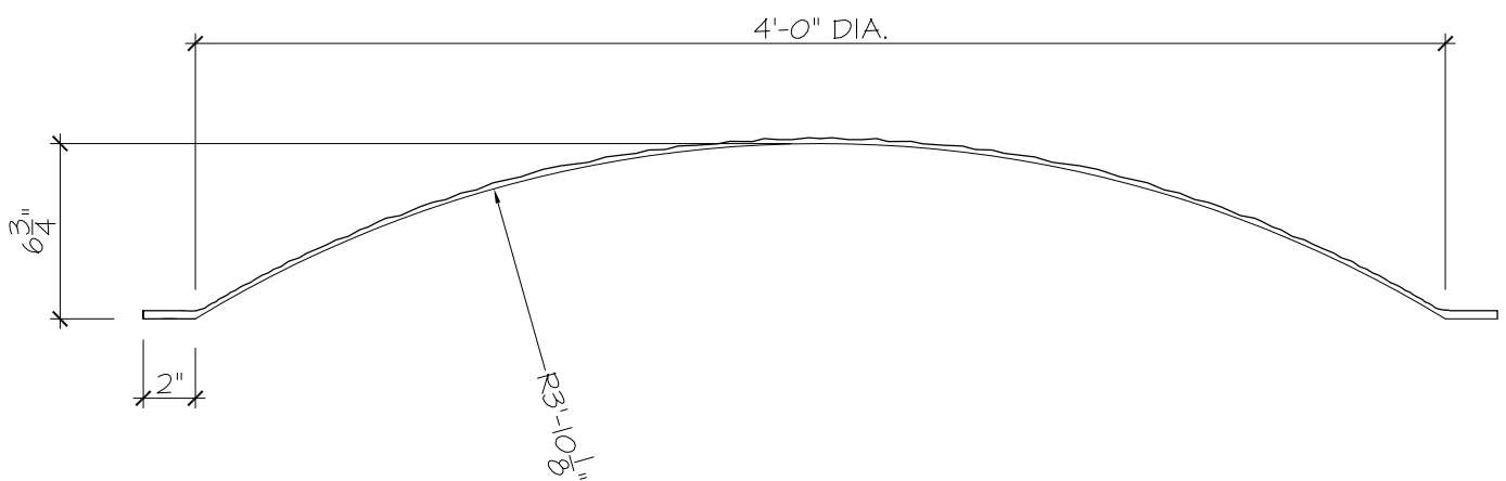
1B DETAIL SECTION SCALE : 1-1/2" = 1'-0"
