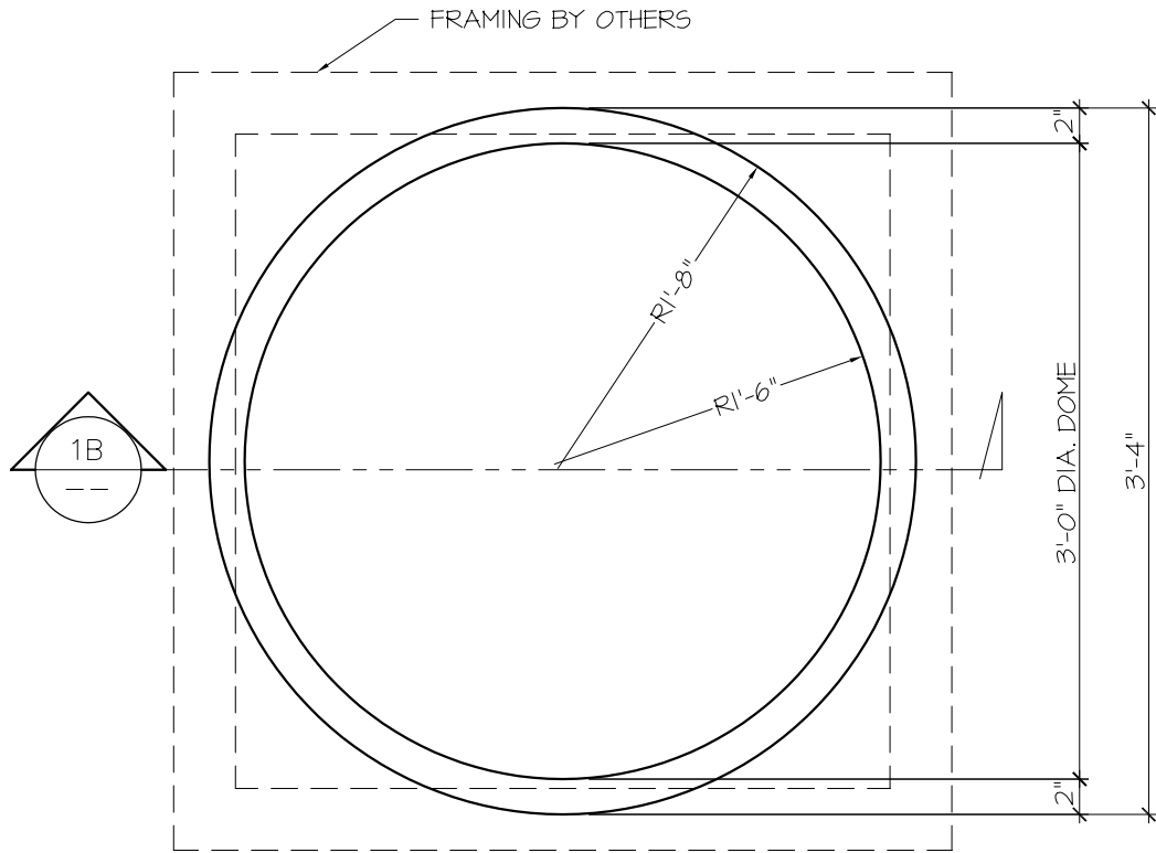
1A REFLECTED PLAN VIEW SCALE : 1" = 1'-0"
