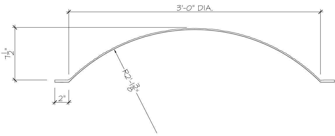
1B DETAIL SECTION SCALE : 1-1/2" = 1'-0"
